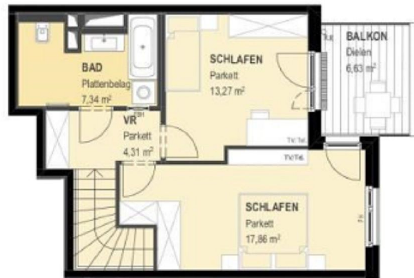
1. Stock
